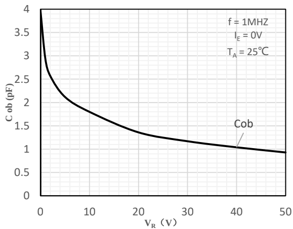
Fig 5 Output Capacitance
