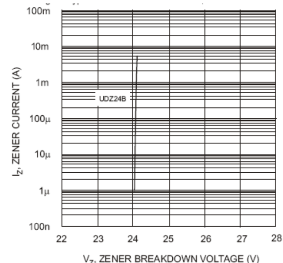
Fig. 6 Typical Reverse Characteristics, UDZ24B
