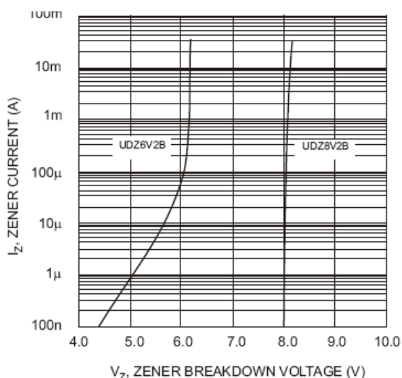
Fig. 3 Typical Reverse Characteristics, UDZ6V2B - UDZ8V2B
