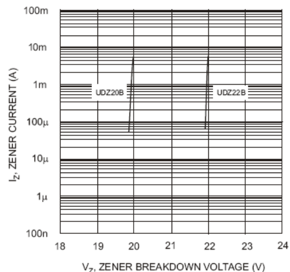
Fig. 5 Typical Reverse Characteristics, UDZ20B - UDZ22B
