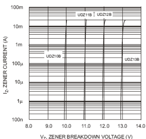
Fig. 4 Typical Reverse Characteristics, UDZ10B - UDZ13B
