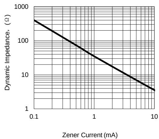
Fig.2 Z z -I z Characteristics
