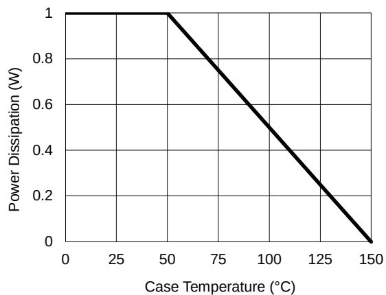
Fig.1 Power Dissipation
