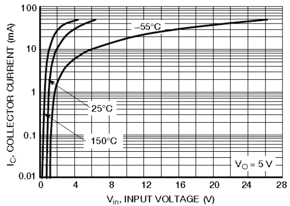
Figure 4. Output Current vs. Input Voltage
