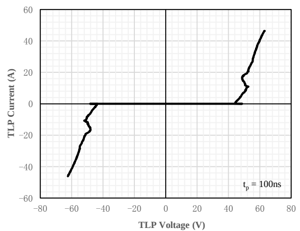
Fig 6 TLP Measurement
