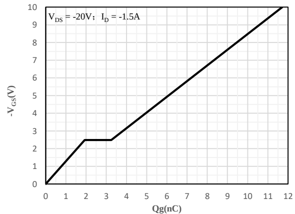
Fig 10 Gate-Charge Characteristics
