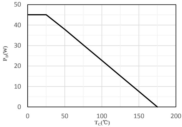
Fig 1 Power Dissipation
