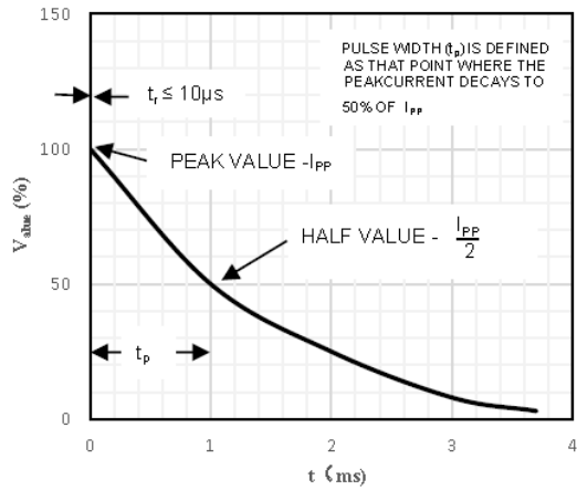
Fig 7 Pulse Waveform
