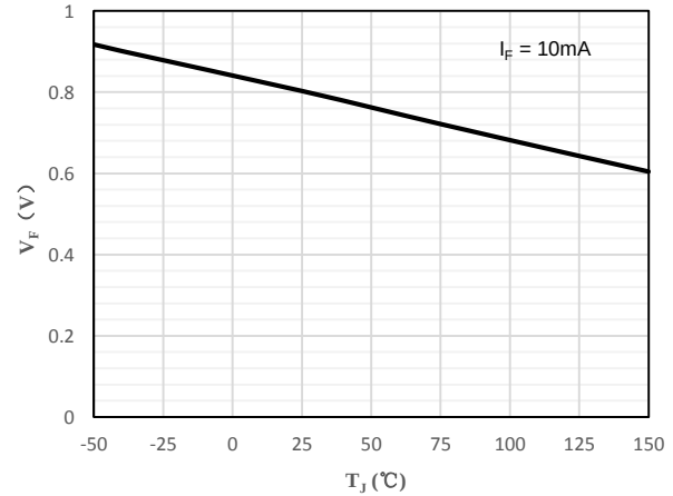
Fig 4 Typical Forward Voltage vs. Temperature
