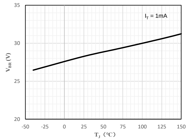
Fig 2 Typical Breakdown Voltage vs. Temperature
