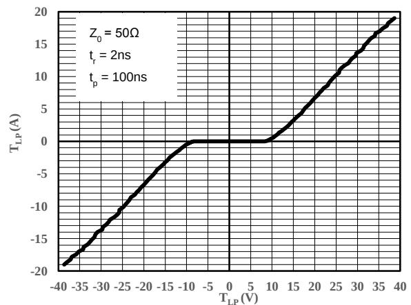
Fig 4 TLP Measurement
