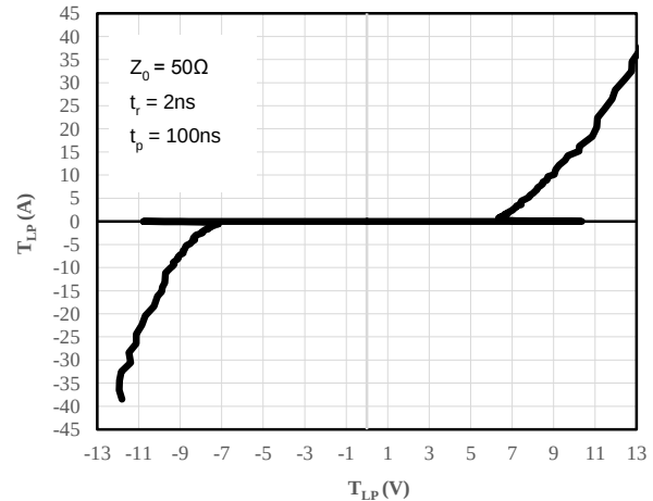
Fig 4 TLP Measurement
