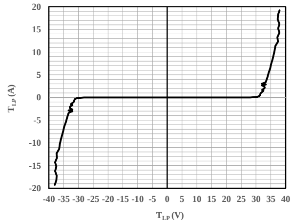
Fig 6 TLP Measurement
