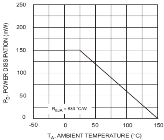
Fig. 1 Derating Curve
