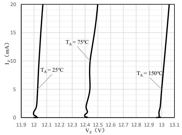
Fig 2 Typical Zener Breakdown
