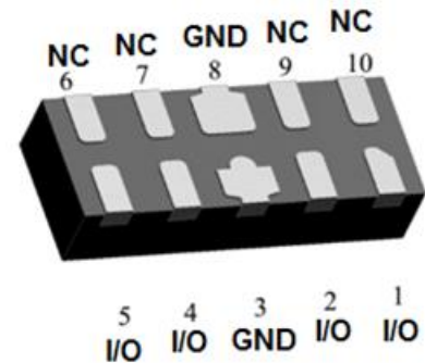
DFN2510-10L
