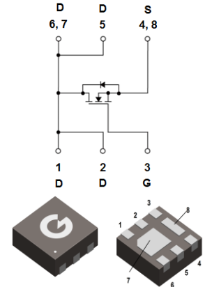
DFN2020-6L
