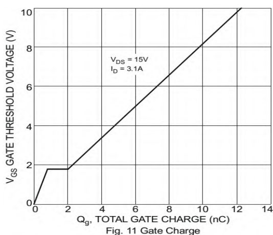
Fig. 11 Gate Charge
