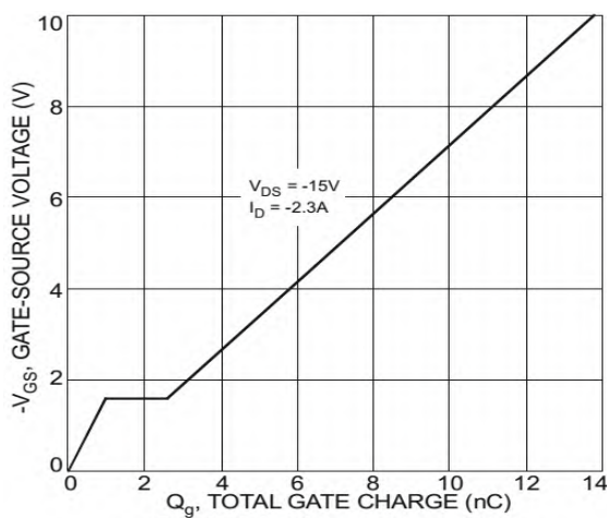
Fig. 23 Gate-Charge Characteristics
