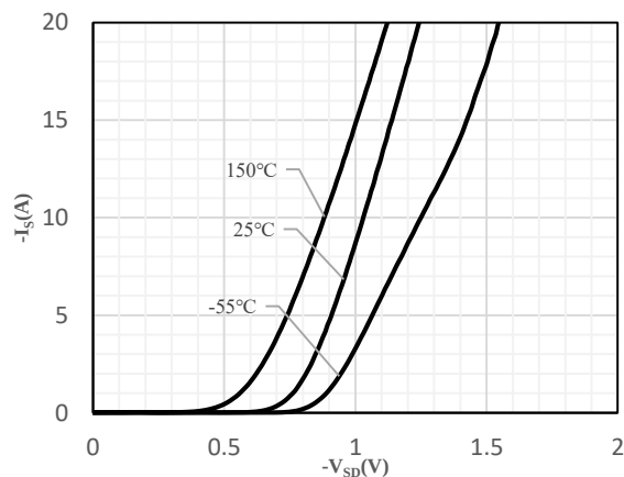
Fig 6 Body-Diode Characteristics
