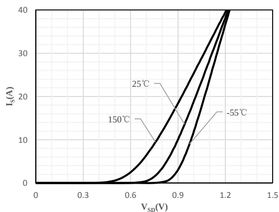
Fig 6 Body-Diode Characteristics
