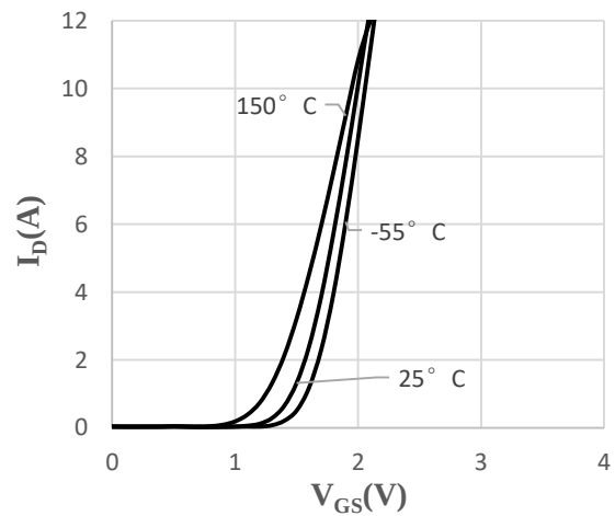
Fig 6 Transfer Characteristics
