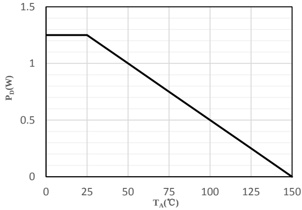
Fig 1 Power Dissipation
