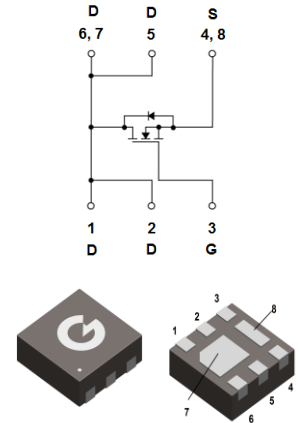
DFN2020-6L
