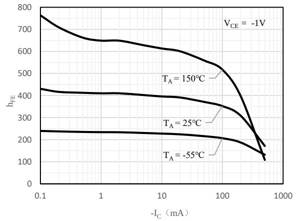
Fig 2 h_{FE} vs. I_C (TBCW67B)
