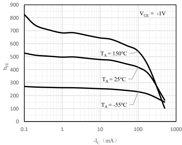
Fig 3 h_{FE} vs. I_C (TBCW67C)
