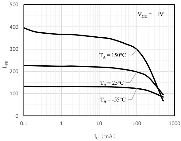
Fig 1 h_{FE} vs. I_C (TBCW67A)
