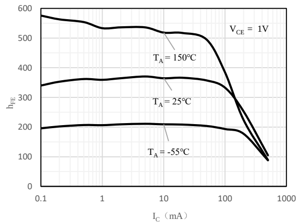
Fig 2 h_{FE} vs. I_C (TBCW66G)
