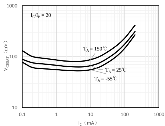
Fig 2 V_{CE(sat)} vs. I_C
