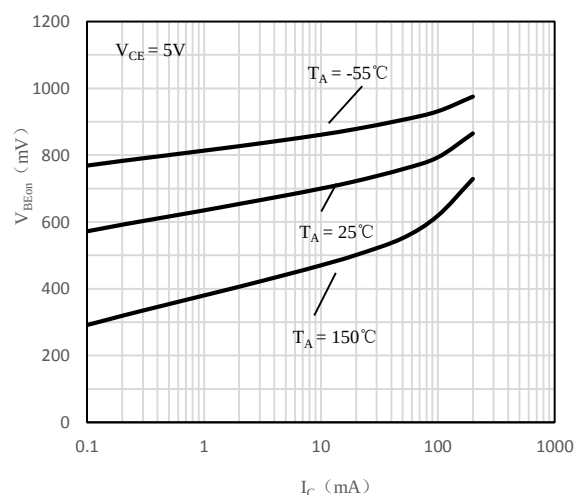
Fig 4 V_{BE(on)} vs. I_C
