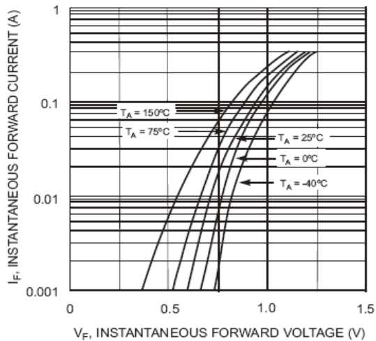
Fig. 1 Forward Characteristics
