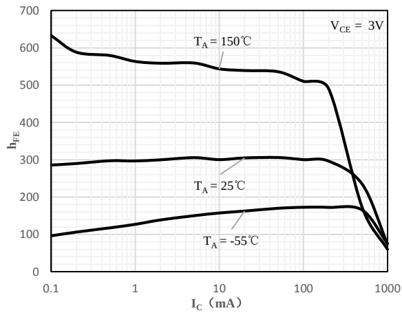
Fig 1 h_{FE} vs. I_C (R:180-390)
