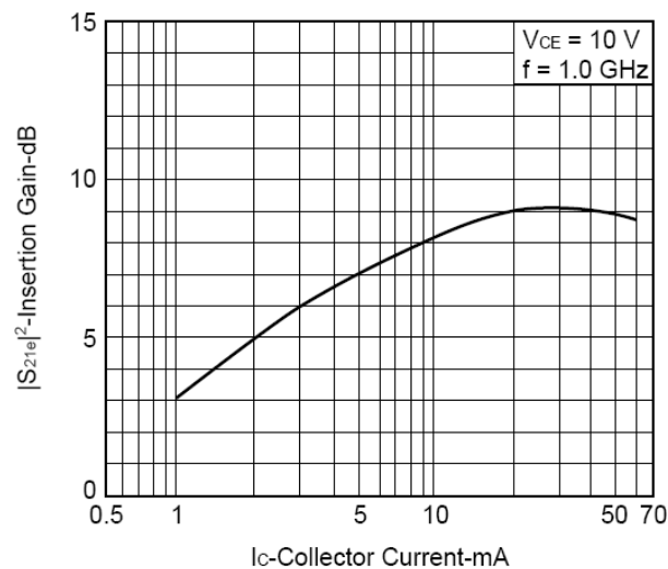
Fig.4 INSERTION GAIN vs. COLLECTOR CURRENT
