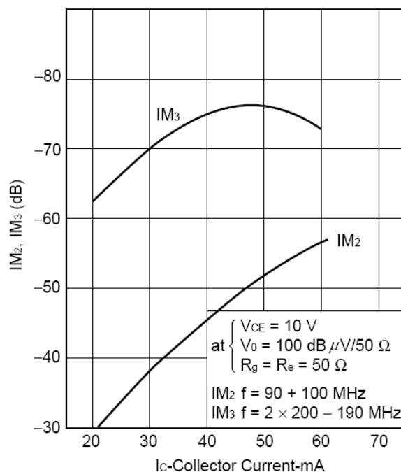
Fig.8 INTERMODULATION DISTORTION vs. COLLECTOR CURRENT
