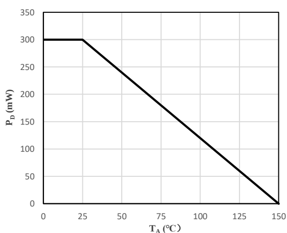
Fig 6 Steady State Power Derating
