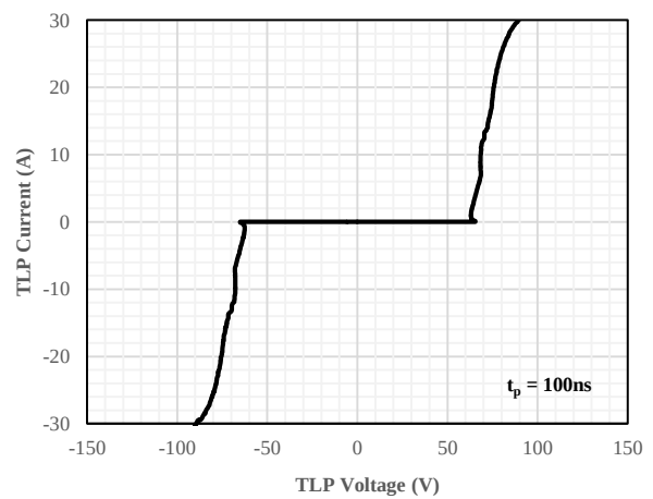
Fig 6 TLP Measurement
