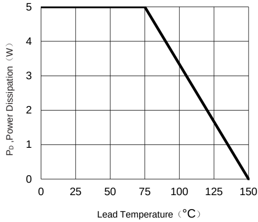
Fig.1 Steady-State Power Derating Curve
