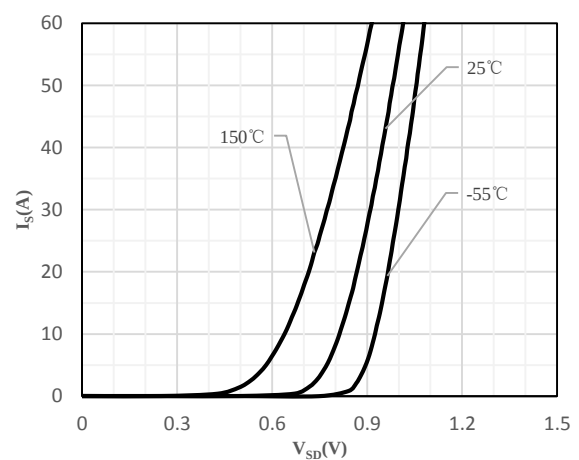
Fig 6 Body-Diode Characteristics
