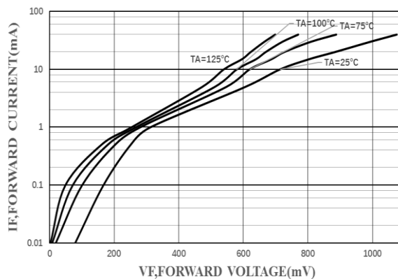
FIG 2.TYPICAL FORWARD CHARACTERISTIC
