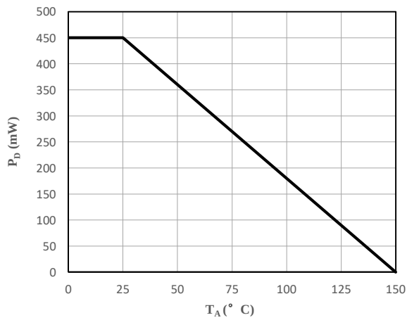
Fig 5 P_D vs. T_A
