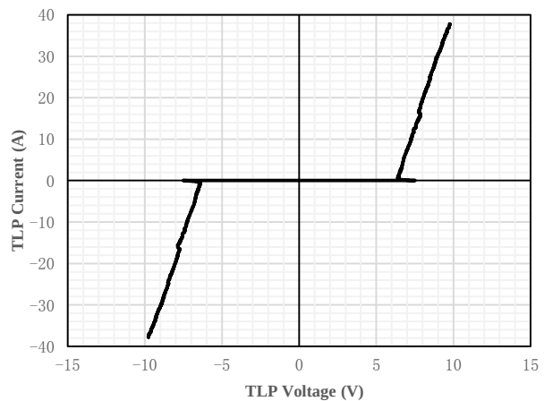
Fig 6 TLP Measurement
