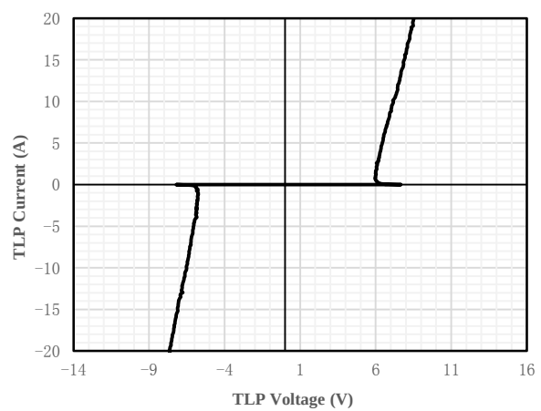
Fig 6 TLP Measurement
