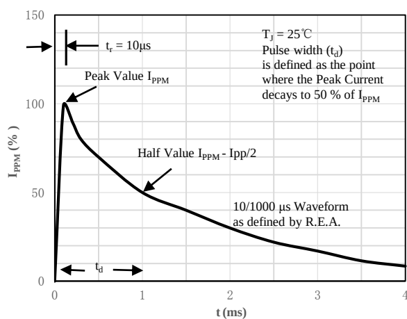
Fig 2 Pulse Waveform
