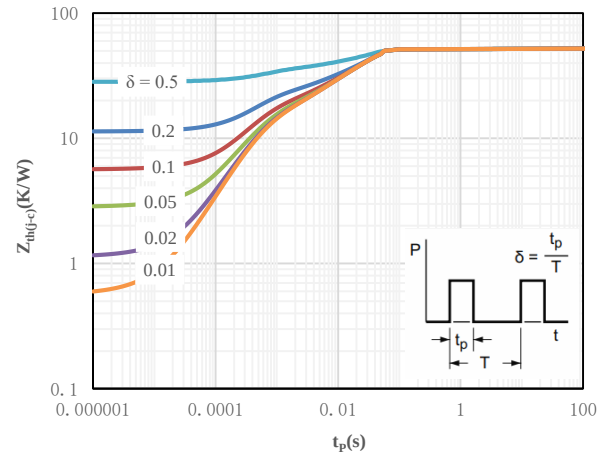
Fig 6 Maximum transient thermal impedance
