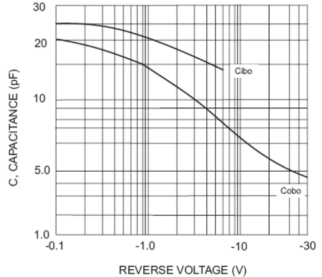
Fig. 2, Capacitances (Typical)
