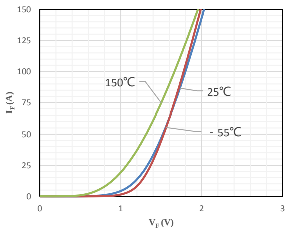
Fig 5 Body-Diode Characteristics
