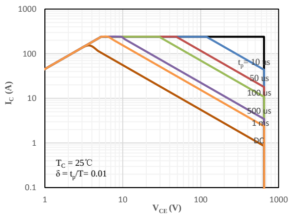
Fig 13 SOA characteristics
