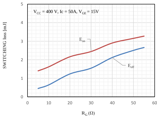
Fig 11 Switching Loss vs. Gate Resistor
