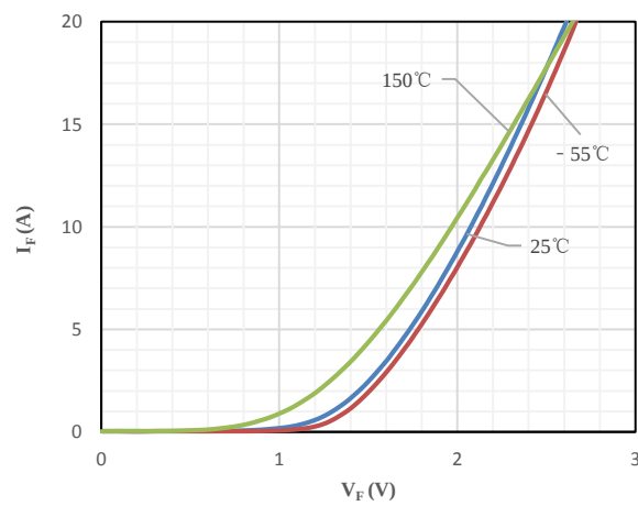
Fig 5 Body-Diode Characteristics
