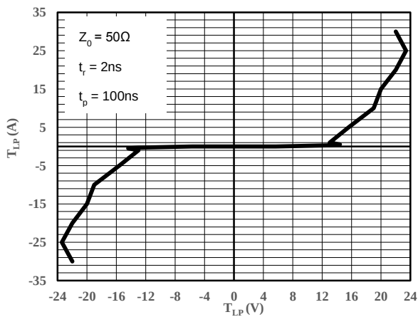
Fig 5 TLP Measurement
