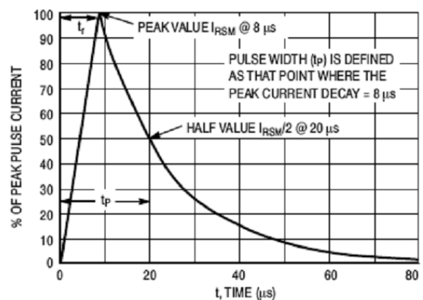
Figure 4. 8 \times 20 \mu\text{s} Pulse Waveform
