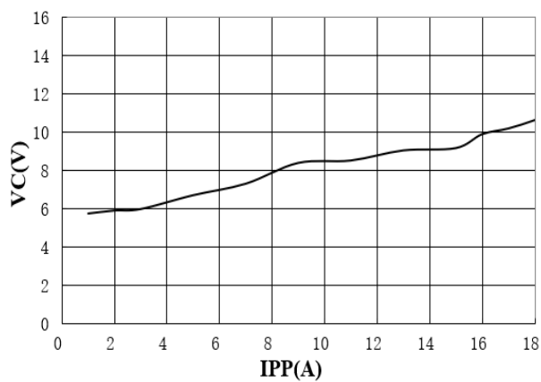
Fig3. IPP VS VC Curve
