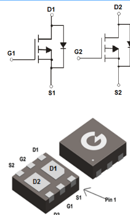
DFN2020-6LC
