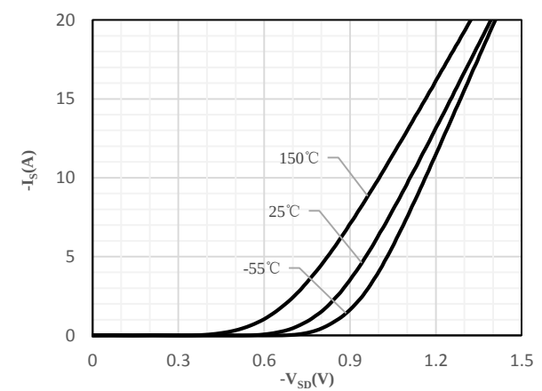
Fig 6 Body-Diode Characteristics
