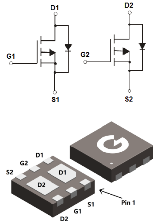
DFN2020-6LC
