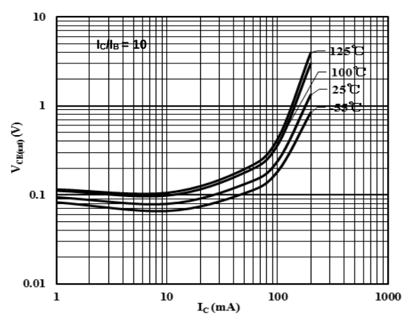
Fig 4 V_{CE(sat)} vs. I_C
