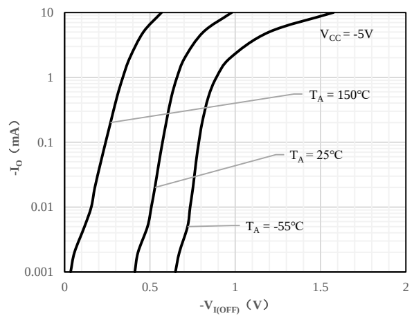
Fig 4 Output Current vs Input Voltage
